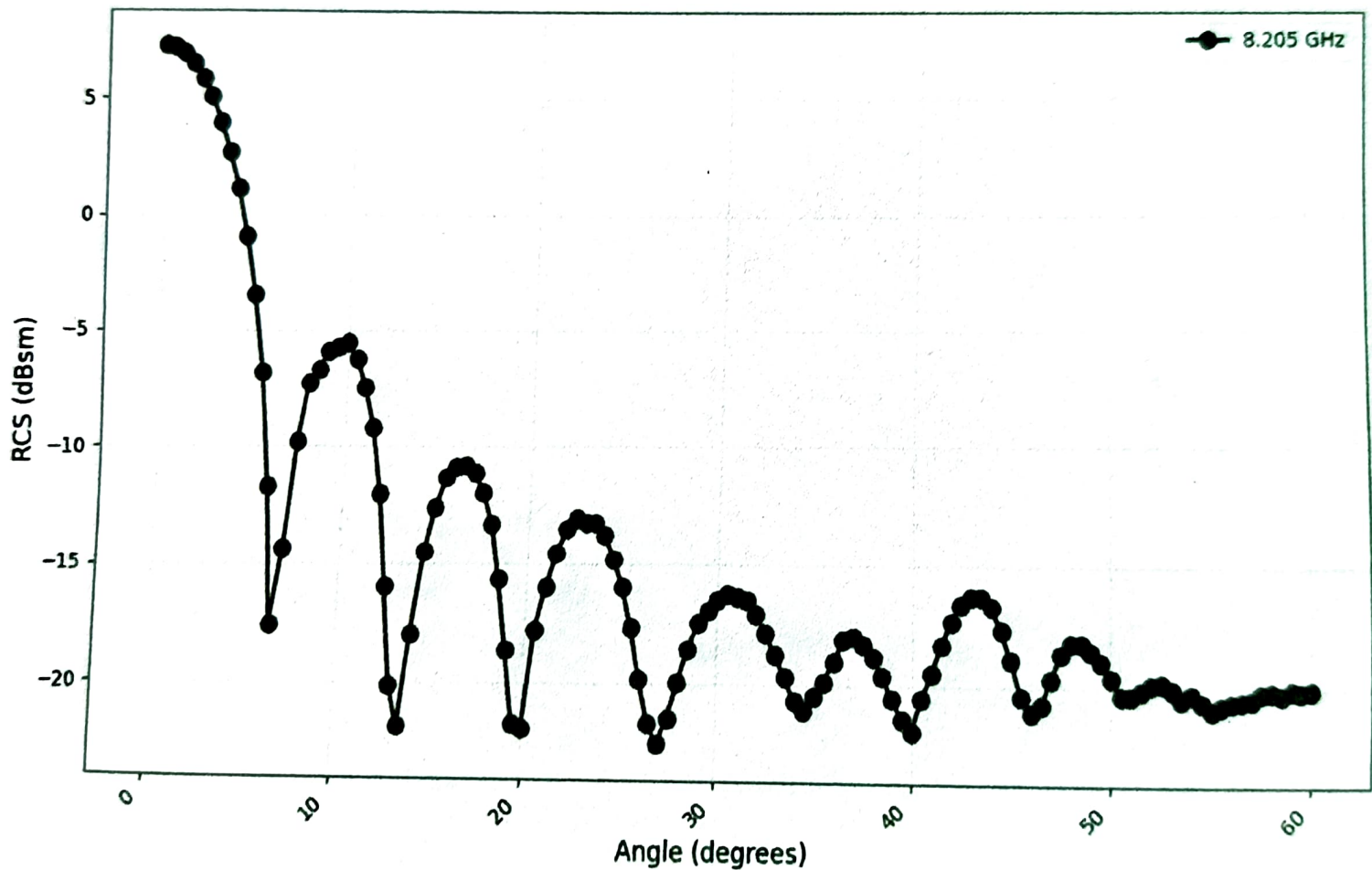
RCS vs Angle at 8.205 GHz
